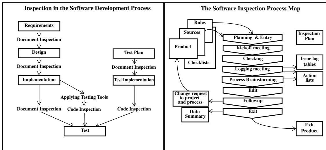
Figure 1: The the Software Development Process and the Software Inspection Process
